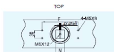
AIR CONNECTION
