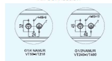
AIR CONNECTION
