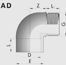
Material PVC-U Thread BSP
