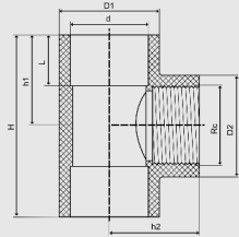
Material PVC-U Thread BSPT
