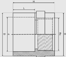
Material PVC-U Thread BSPT
